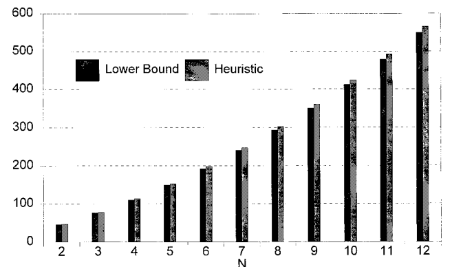
Figure 3. Compound Poisson Examples.
